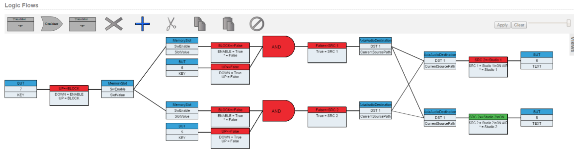
Example of airchain switcher requiring dual button press for safety.
